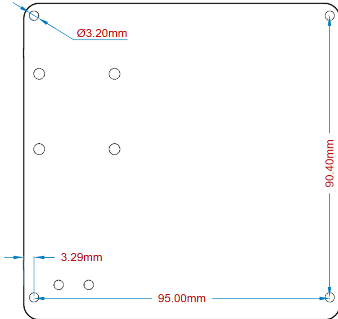
Mounting holes
